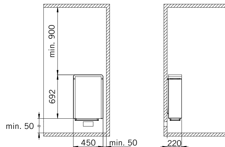
Safety distances for Concept R mini 3.5, 4.5, 6 and 7.5 kW (CP-RM-35 / CP-RM-45 / CP-RM-60 / CP-RM-75)
